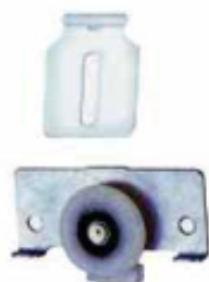
M-688 Adjustable Top & Bottom Roller Set (40kg) Track : M880-1/2
