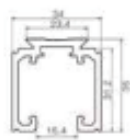
ZY-328 3 meters Track Top & Bottom Track
