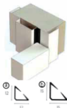
MI-1212 12 x 12 x 2400mm Perimeter Seal Black Door Clearance: 2-3mm
