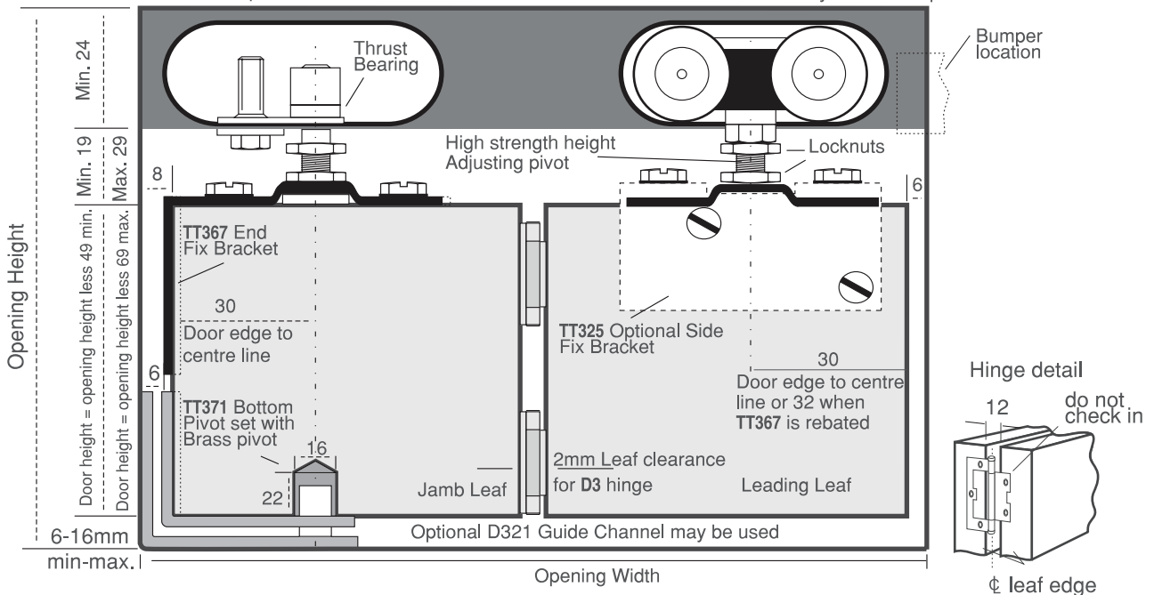
TT370 Top Pivot Set includes End Fix Bracket
