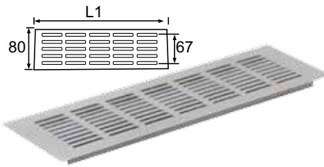
WH-01 L1: 150, 250, 300, 350, 400, 450, 500, 600mm Aluminium Ventilator
